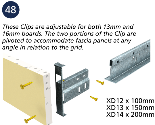
■ FASCIA TRIM CLIPS & TYPICAL APPLICATION
