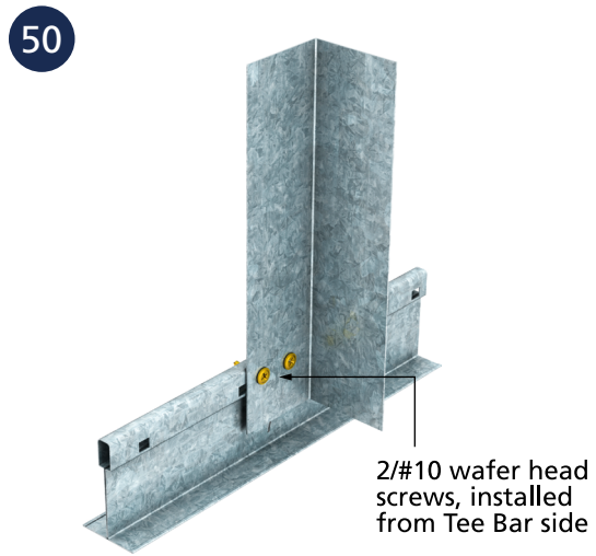
■ SA12 SECURED TO WEB
